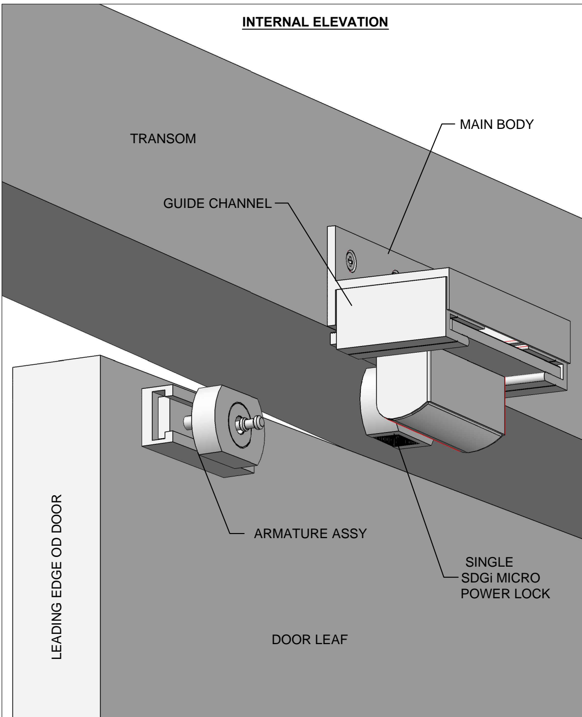
SDGI SINGLE MICRO POWER LOCK BRACKET ASSEMBLED DETAIL
