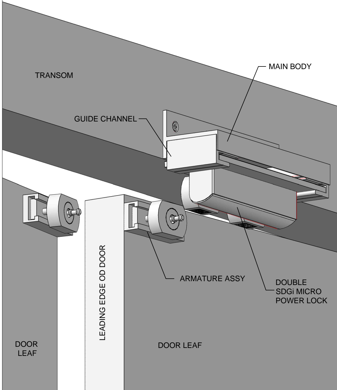
SDGI DOUBLE MICRO POWER LOCK BRACKET ASSEMBLED DETAIL
