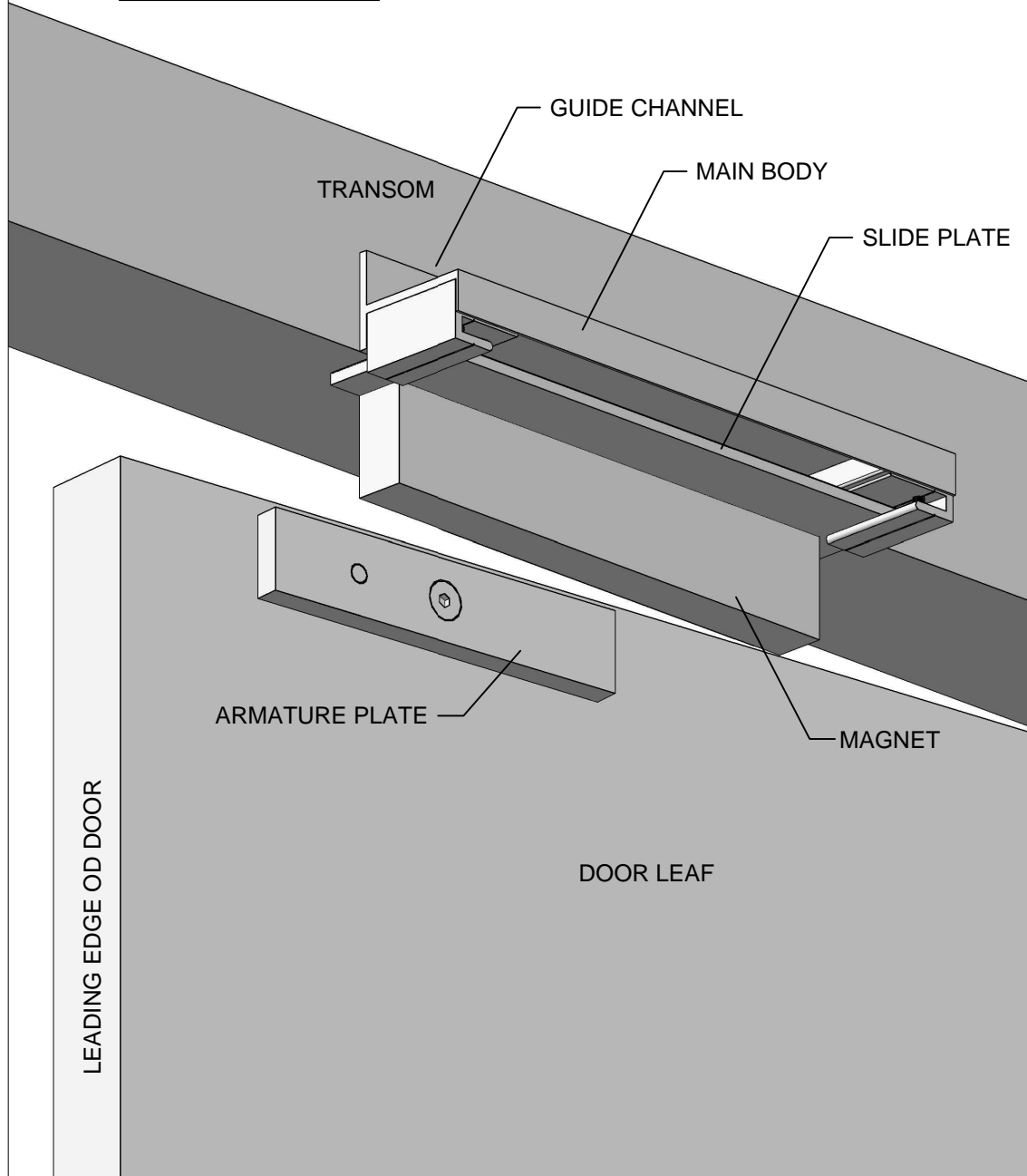
SDGI BRACKET ASSEMBLED DETAIL
